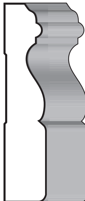
954 3/4" x 3 1/2"
