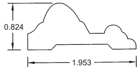
2" PANEL MOULD BL52
