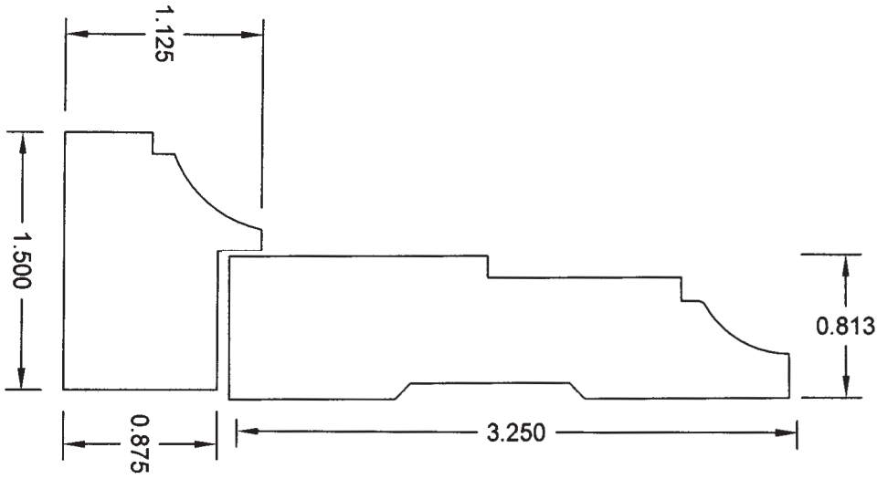
3 1/4" COVE CASE BL25
