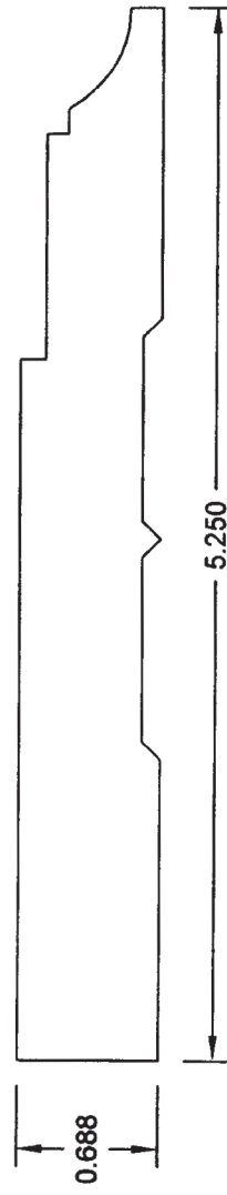
5 1/4" COVE BASE BL28
