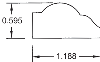
A9 MOULD BL47
