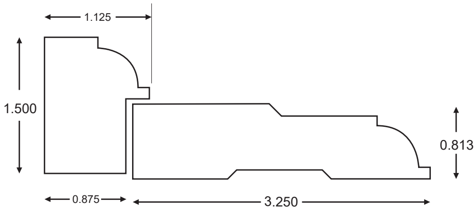
3 1/4" BEAD CASE BL37
