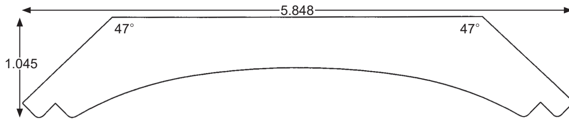
5 7/8" COVE CROWN BL21
