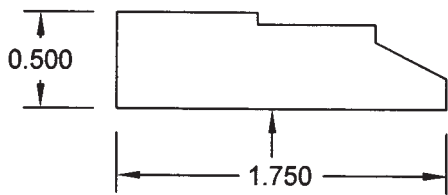
BEVEL STOP & SHOE BL32
