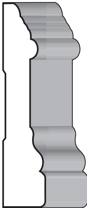
7715 3/4" x 3 1/2"
