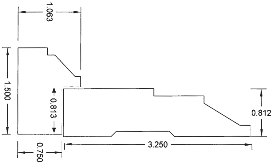
BEVEL STACK BL30 3 1/4" BEVEL CASE BL31
