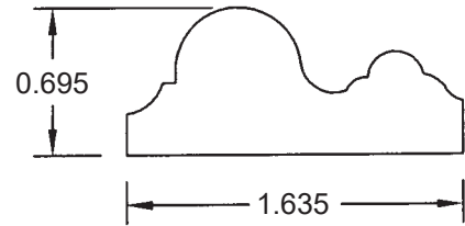
1 5/8" PANEL MOULD BL50
