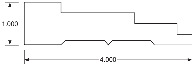
3 STEP CASE BL412
