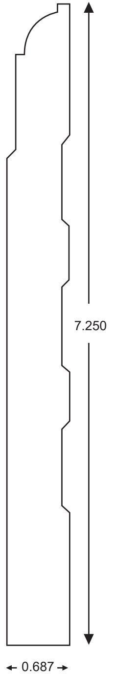
7 1/4" BEAD BASE BL41
