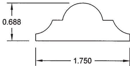
1 3/4" BEAD PANEL MOULD BL48
