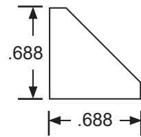
5/8" PANEL MOULD BL415
