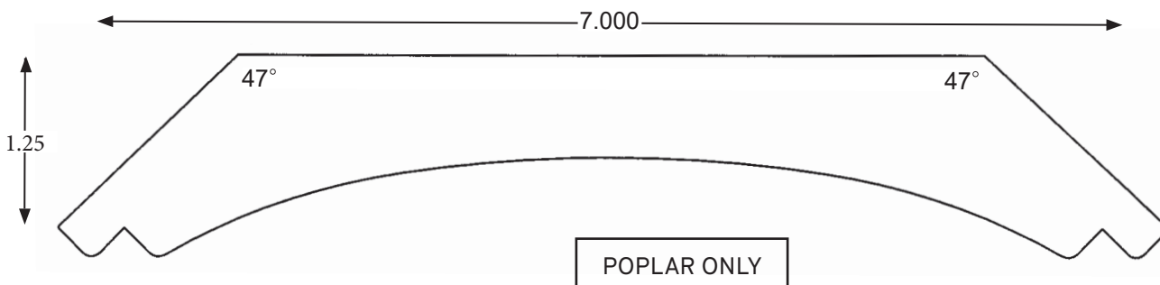
7" COVE CROWN L7PCOVE
