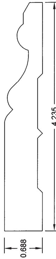
4 1/4" COLONIAL BASE BL5
