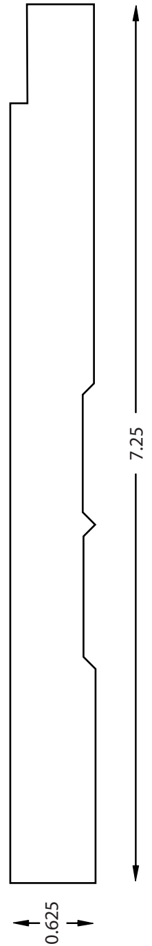
7 1/4" LOFT BASE BL416
