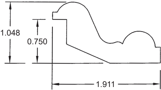
3/4" RAISED PANEL MOULD BL55
