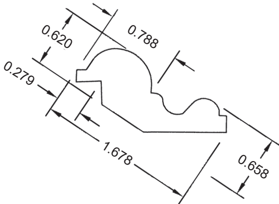
1/2" RAISED PANEL MOULD BL54
