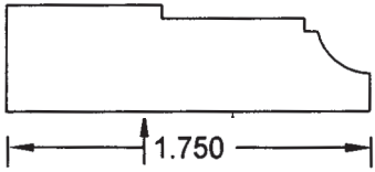
COVE STOP & SHOE BL26
