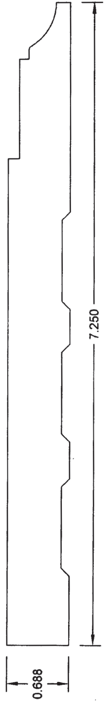
7 1/4" COVE BASE BL29
